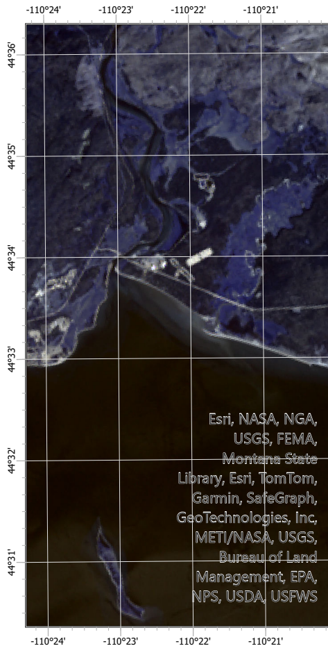
Multispectral
