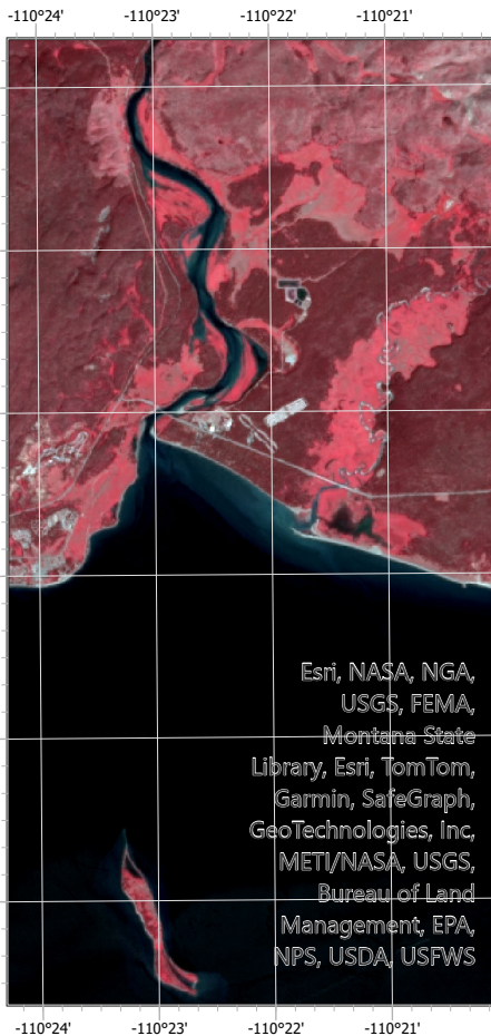
Pan-Sharpended CIR
