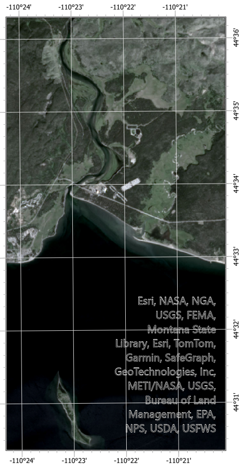
Pan-Sharpended True color
